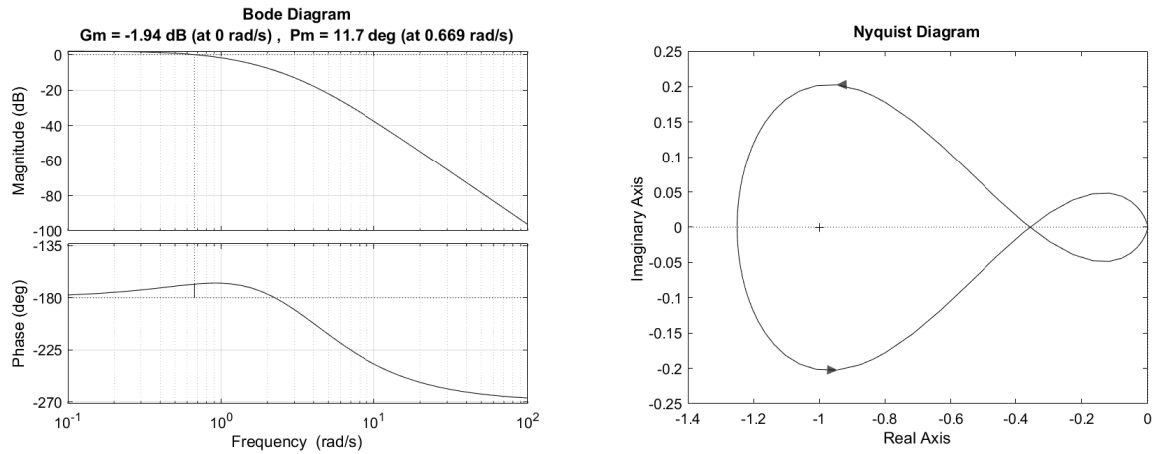
Figure 8.2.3: Bode and Nyquist plot for Example 8.2.8.
