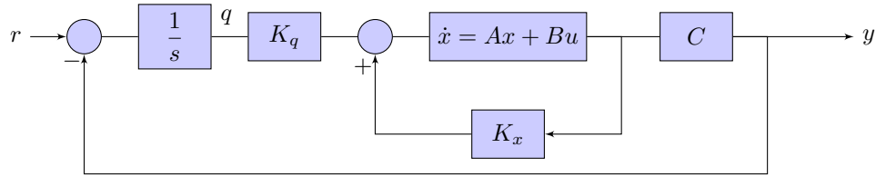
Figure 10.5.1: Full-state feedback with integral action.
