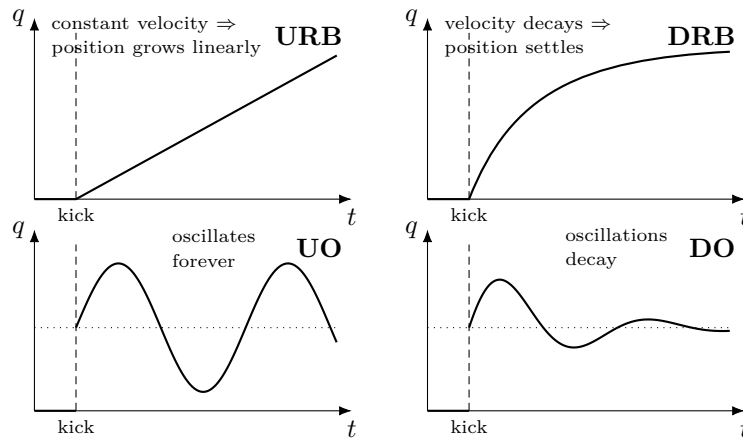
Figure 2.4.1: Qualitative position responses q(t) to a short “kick” starting from zero initial conditions.
