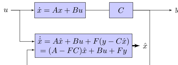
Figure 10.3.1: Output-driven state observer. The observer uses the input u and the output y to compute the state estimate \hat{x} .
