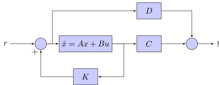
Figure 10.2.1: Full-state feedback control system.
