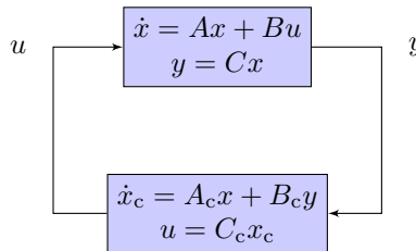
Figure 10.4.1: Dynamic output-feedback controller. The controller uses the measured output y to generate the control input u through the controller state x_c .
