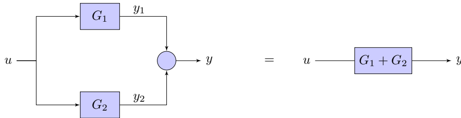
Figure 7.1.4: Parallel connection.
