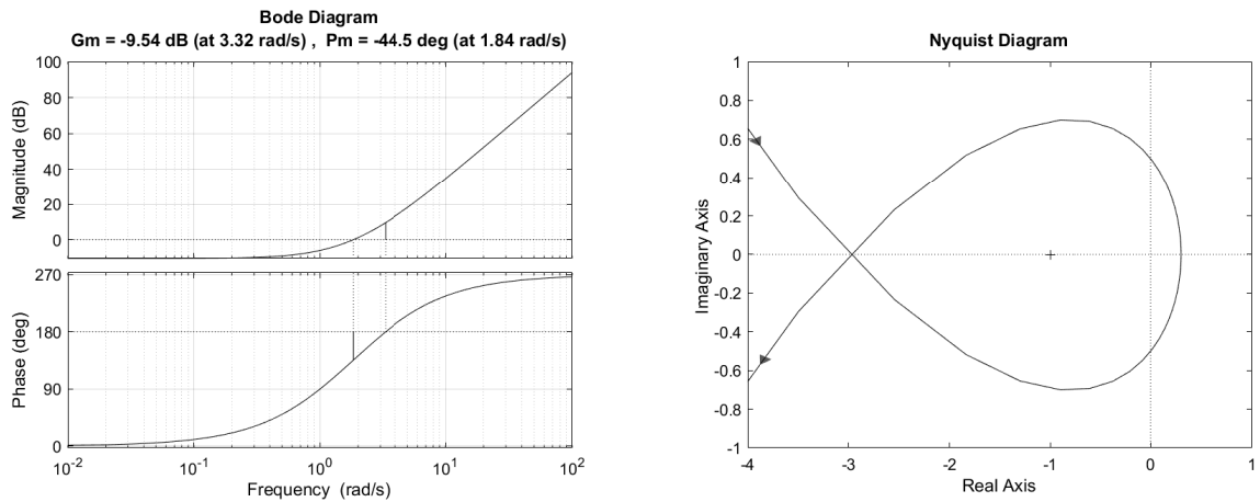
Figure 8.2.4: Bode and Nyquist plot for Example 8.2.9.
