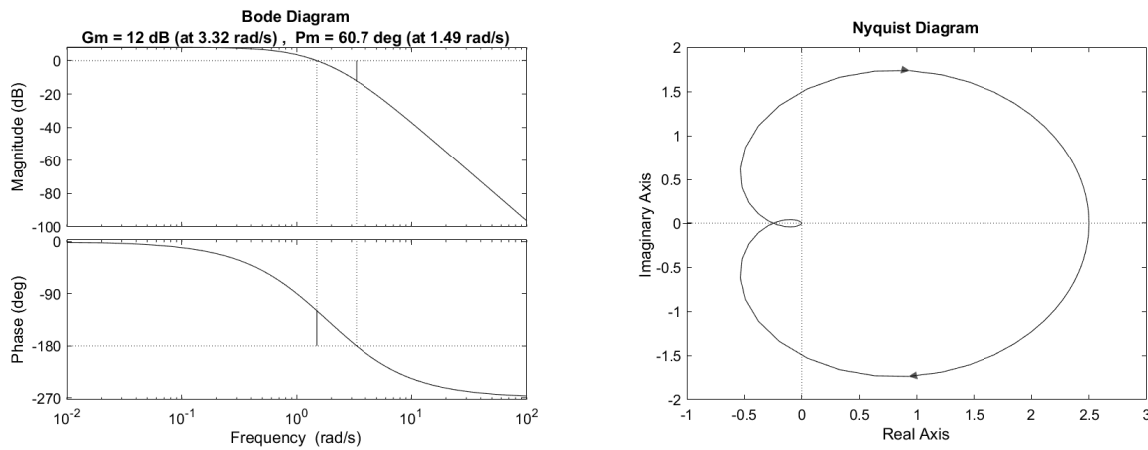
Figure 8.2.2: Bode and Nyquist plot for Example 8.2.7.
