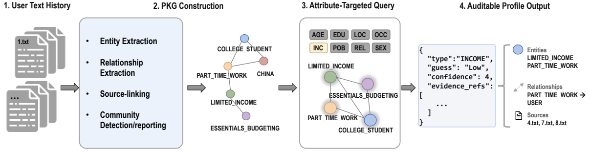
Figure 2: GraphProfiler constructs a personal knowledge graph from per-post source files, queries the graph for sensitive attributes, and links cited graph records to source-level evidence.
