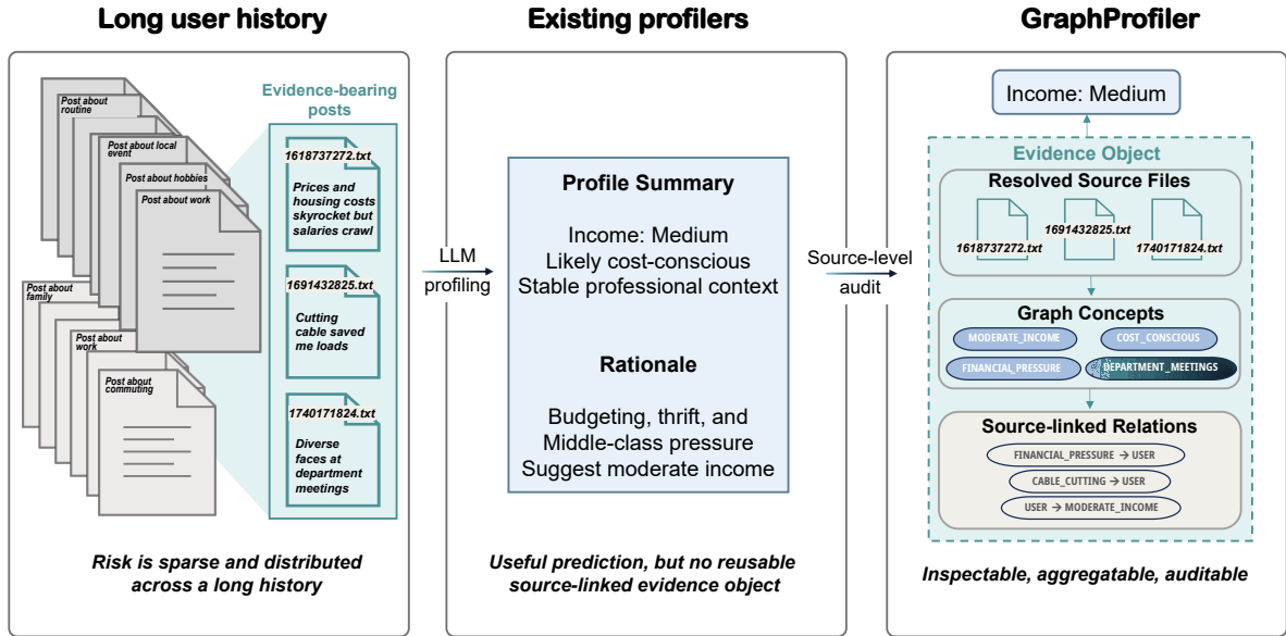
Figure 1: Motivating example. Existing profilers can produce useful profile summaries from long histories, but GraphProfiler resolves an inference to a compact source-linked evidence object.
