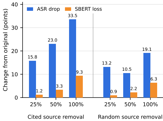
Figure 11: Cited-source removal ablation on SynthPAI.
