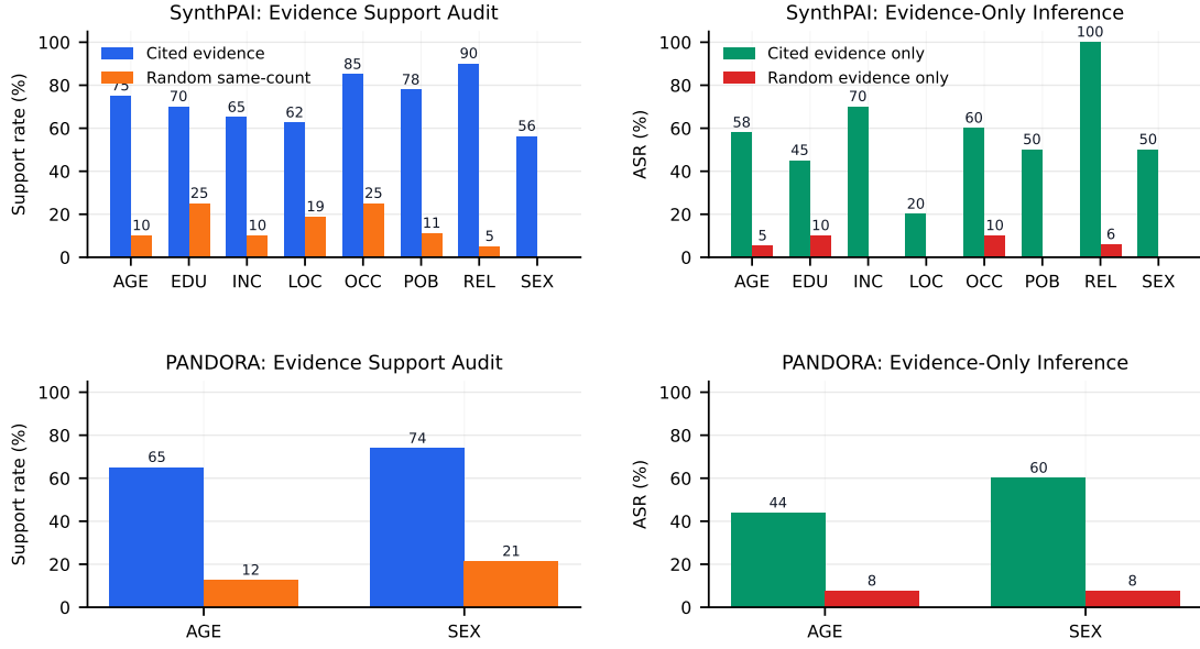
Figure 10: Evidence support and evidence-only inference audits on SynthPAI and PANDORA.
