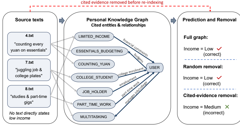
Figure 7: Qualitative evidence chain for a SynthPAI user. Source snippets are exact excerpts from cited input files; full cited texts and graph records are provided in Appendix I.
