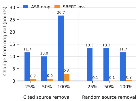
Figure 5: Cited-source removal ablation on PANDORA.
