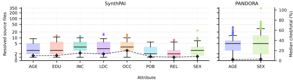
Figure 9: Resolved source files cited per prediction on SynthPAI and PANDORA. Dashed diamonds show the median cited/total source-file ratio.
