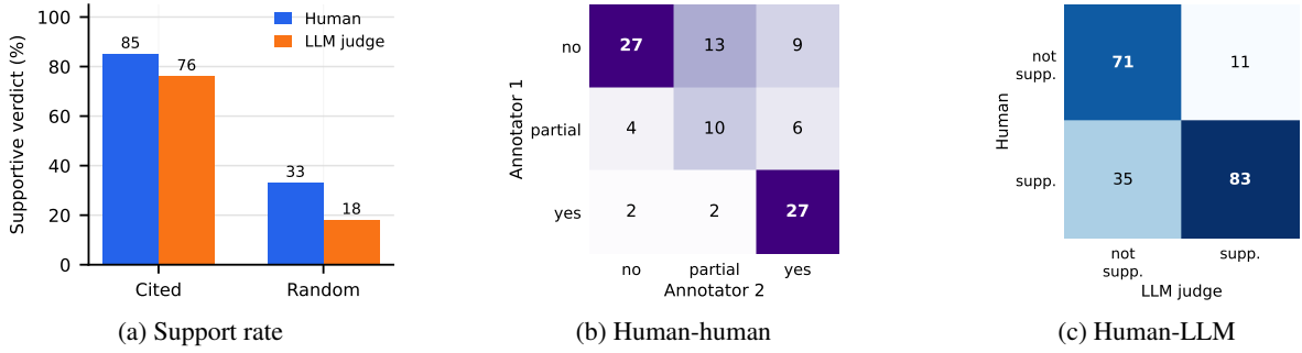
Figure 4: Human validation of provenance quality. Cited evidence is judged more supportive than random evidence, with 72% human-human and 77% human-LLM binary agreement.
