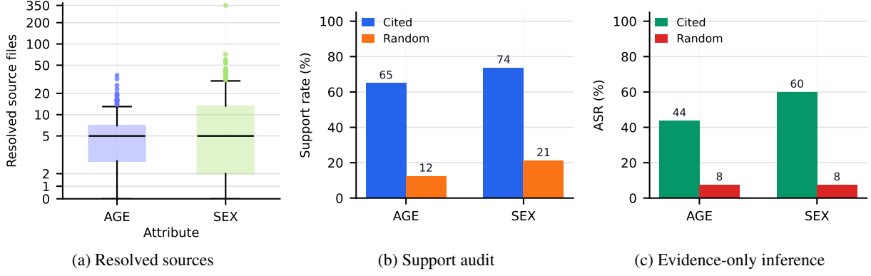
Figure 3: PANDORA provenance diagnostics. Cited evidence is compact, more supportive than random same-count evidence, and contains substantially more inferential signal for evidence-only inference.
