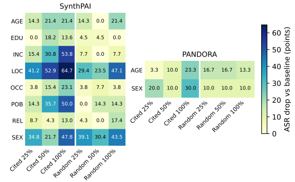
Figure 12: Attribute-wise ASR drop under cited-source removal. Columns show cited-source removal and random same-count source removal at 25%, 50%, and 100%; values are point drops relative to the original graph condition.
