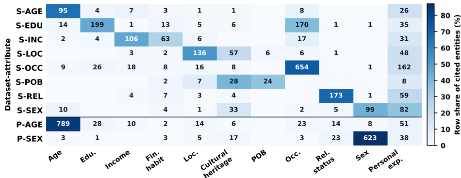
Figure 6: Directly cited graph entity types by inferred attribute on SynthPAI (S) and PANDORA (P). Cell values are raw cited-entity counts, and normalized colors within each row show the dominant entity types for each attribute.
