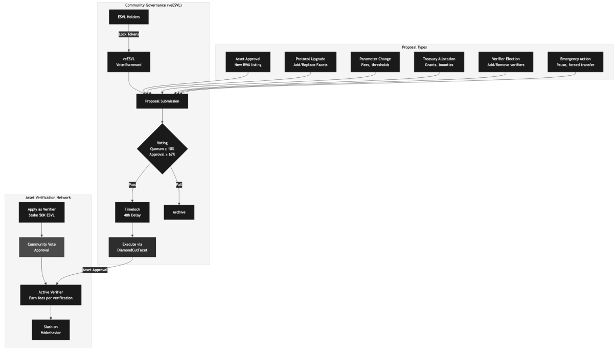
Figure 3: Governance and verification flow. ESVL holders lock tokens to obtain veESVL voting power. Six proposal types cover asset approvals, protocol upgrades, parameter changes, treasury allocation, verifier elections, and emergency actions. The Asset Verification Network operates through staked verifiers elected by community vote.
