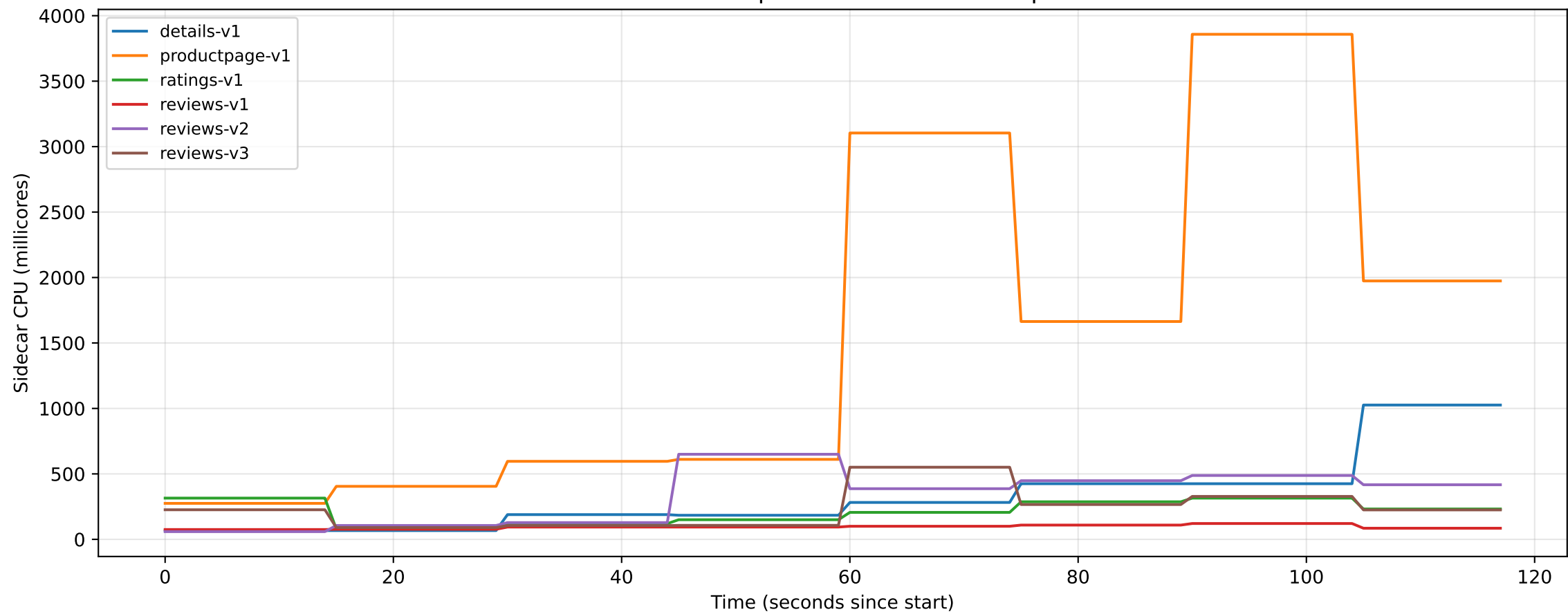
Sidecar CPU per Service — st5-AttUpd
