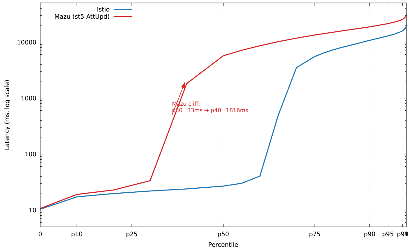
Latency CDF at 400 RPS (run 05-24 20:09:48)
