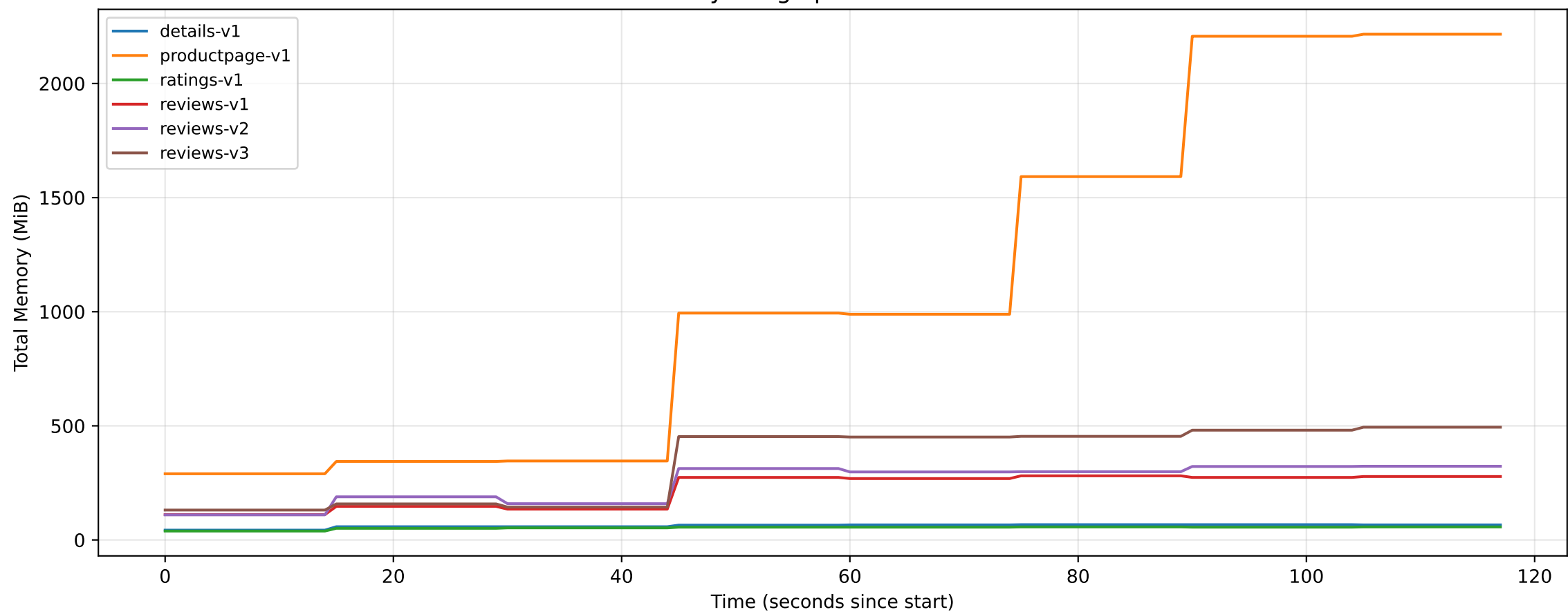
Memory Usage per Service — st5-AttUpd
