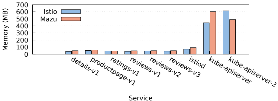
Memory Usage: Istio vs Mazu (200 QPS)
