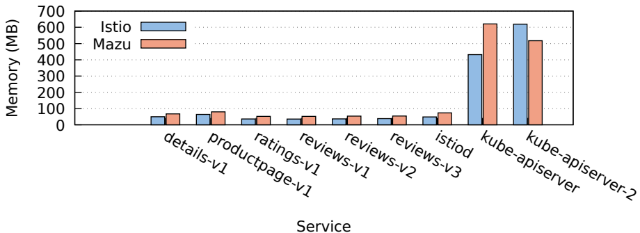
Memory Usage: Istio vs Mazu (600 QPS)
