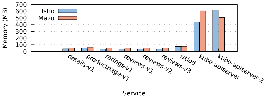
Memory Usage: Istio vs Mazu (300 QPS)
