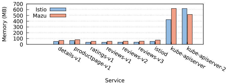
Memory Usage: Istio vs Mazu (700 QPS)
