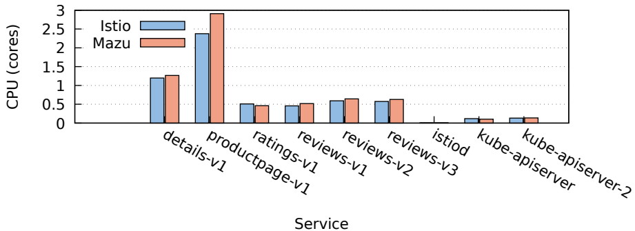
CPU Usage: Istio vs Mazu (300 QPS)
