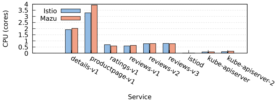
CPU Usage: Istio vs Mazu (400 QPS)
