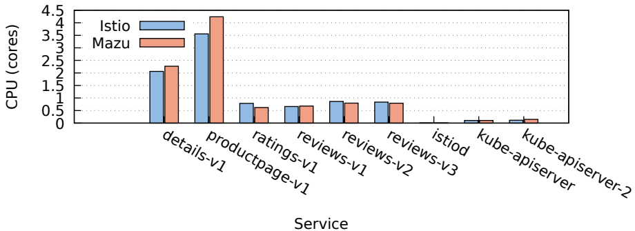
CPU Usage: Istio vs Mazu (600 QPS)
