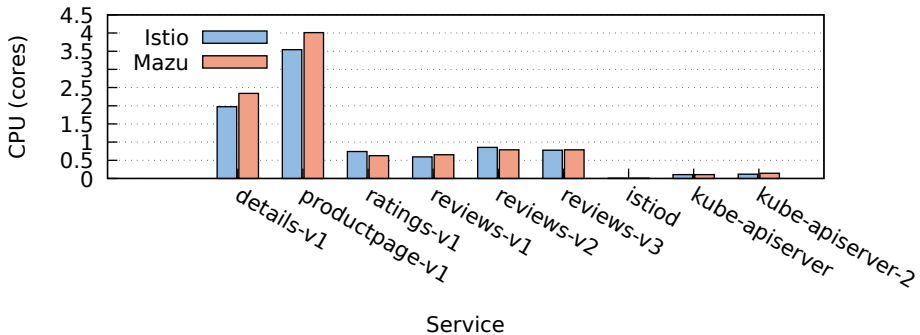
CPU Usage: Istio vs Mazu (800 QPS)
