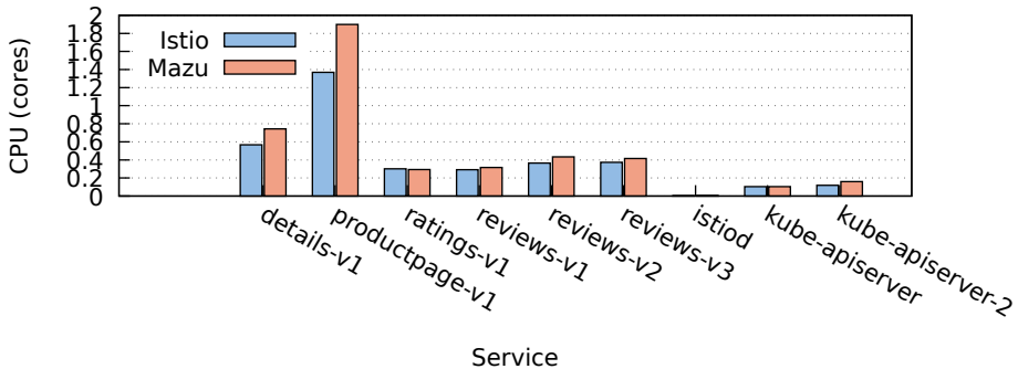
CPU Usage: Istio vs Mazu (200 QPS)
