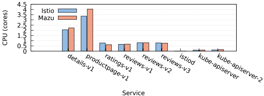
CPU Usage: Istio vs Mazu (700 QPS)
