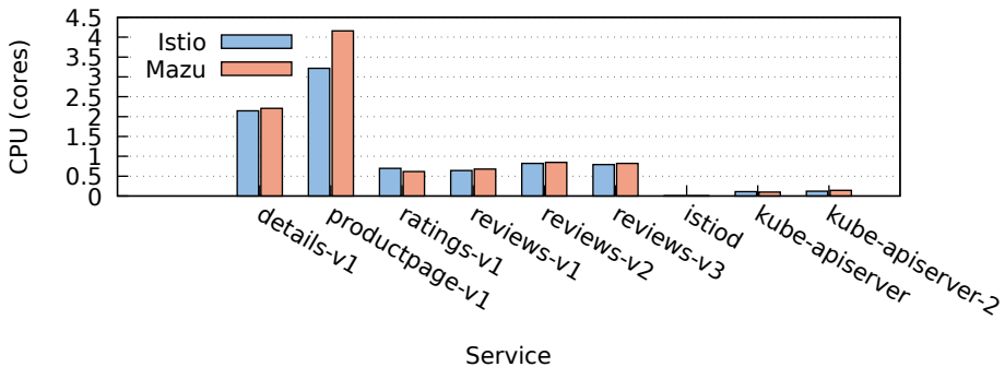
CPU Usage: Istio vs Mazu (500 QPS)
