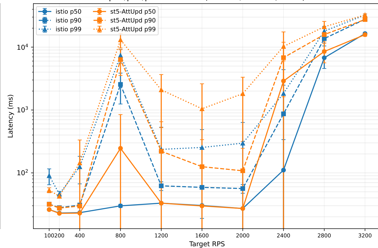
p50/p90/p99 combined (mean +/- stddev, n=10)
