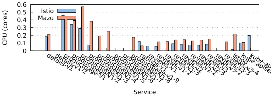
CPU Usage: Istio vs Mazu (500 QPS)
