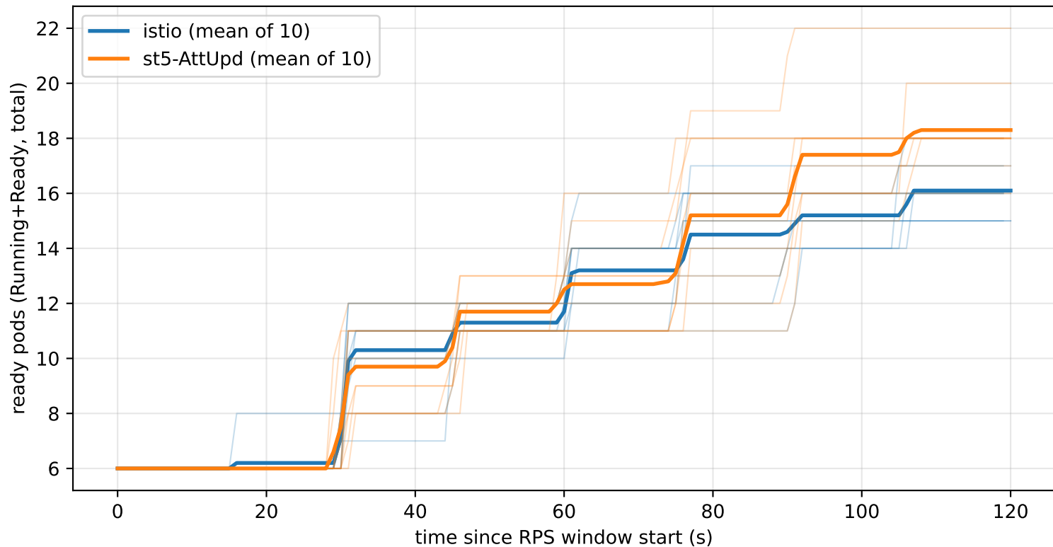
Pod scaling at 400 rps
