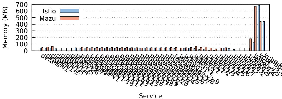
Memory Usage: Istio vs Mazu (700 QPS)
