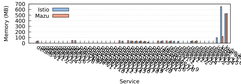
Memory Usage: Istio vs Mazu (300 QPS)
