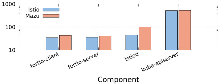
Memory Usage: Istio vs Mazu (50 RPS, 4min)
