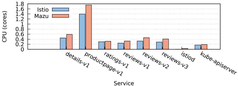
CPU Usage: Istio vs Mazu (80 QPS)
