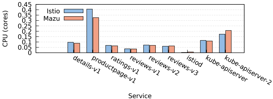
CPU Usage: Istio vs Mazu (150 QPS)
