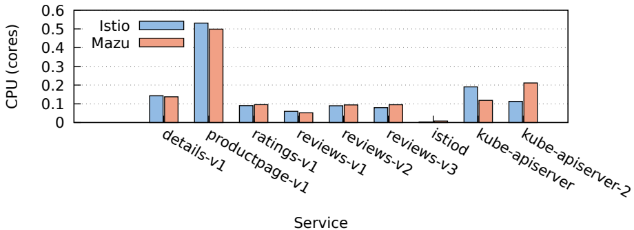
CPU Usage: Istio vs Mazu (250 QPS)
