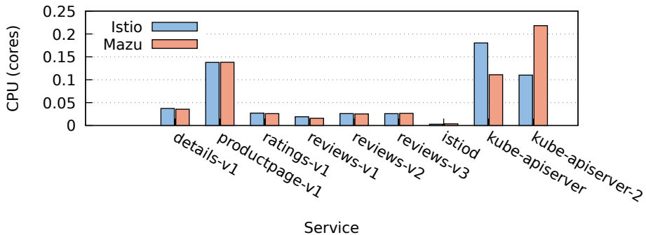
CPU Usage: Istio vs Mazu (50 QPS)
