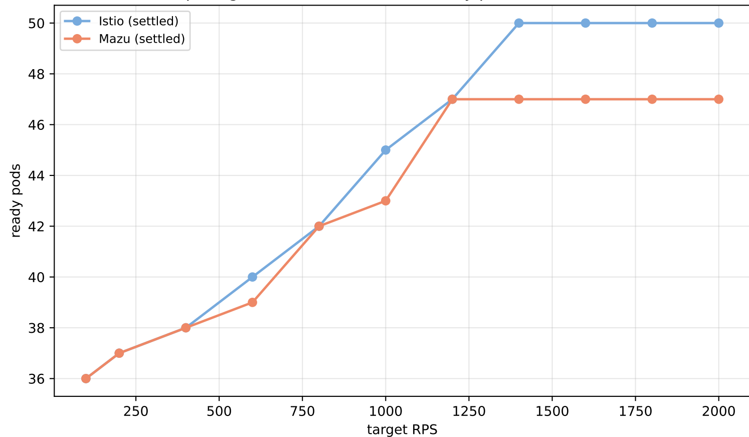
Replica growth under load: total ready pods vs offered RPS
