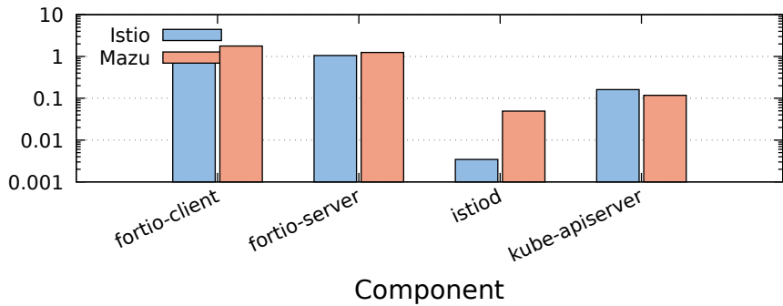
CPU Usage: Istio vs Mazu (50 RPS, 4min)
