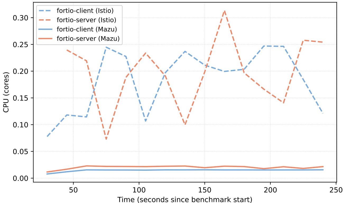
CPU usage over time - application containers
