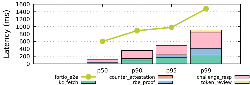
Mazu Latency Breakdown by Operation (50 RPS, 4min)
