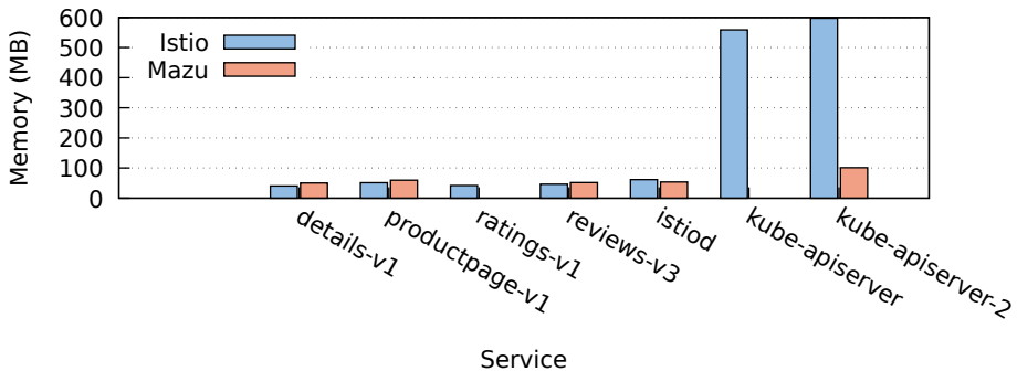
Memory Usage: Istio vs Mazu (20 QPS)
