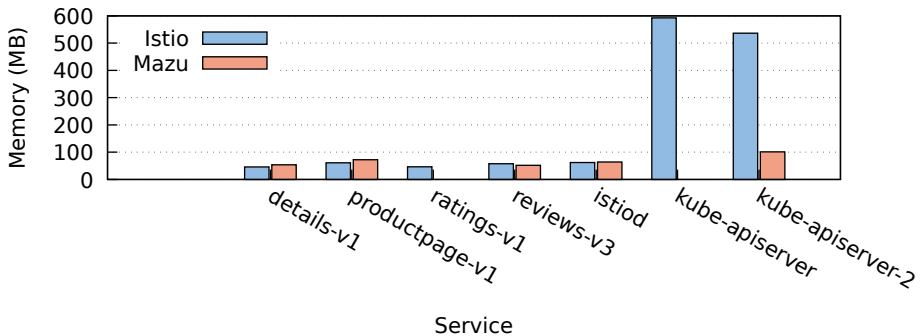
Memory Usage: Istio vs Mazu (80 QPS)
