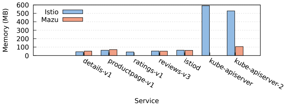
Memory Usage: Istio vs Mazu (60 QPS)
