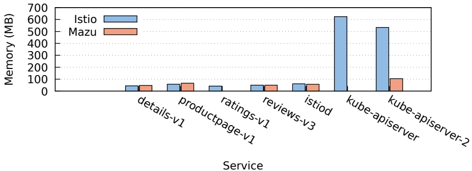
Memory Usage: Istio vs Mazu (40 QPS)
