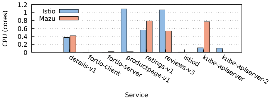
CPU Usage: Istio vs Mazu (40 QPS)
