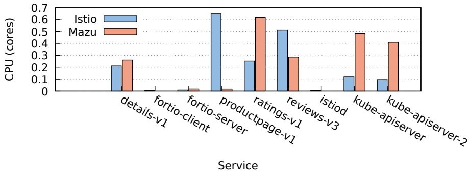
CPU Usage: Istio vs Mazu (20 QPS)
