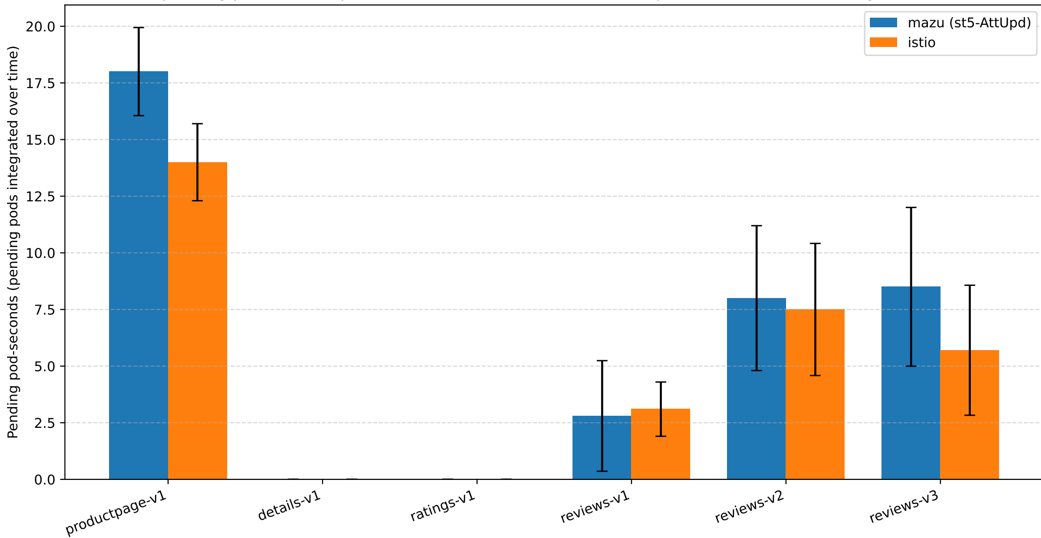
Total pending pod-seconds per service at 300 RPS: mazu (st5-AttUpd) vs istio (mean +/- 1 sigma over runs)
