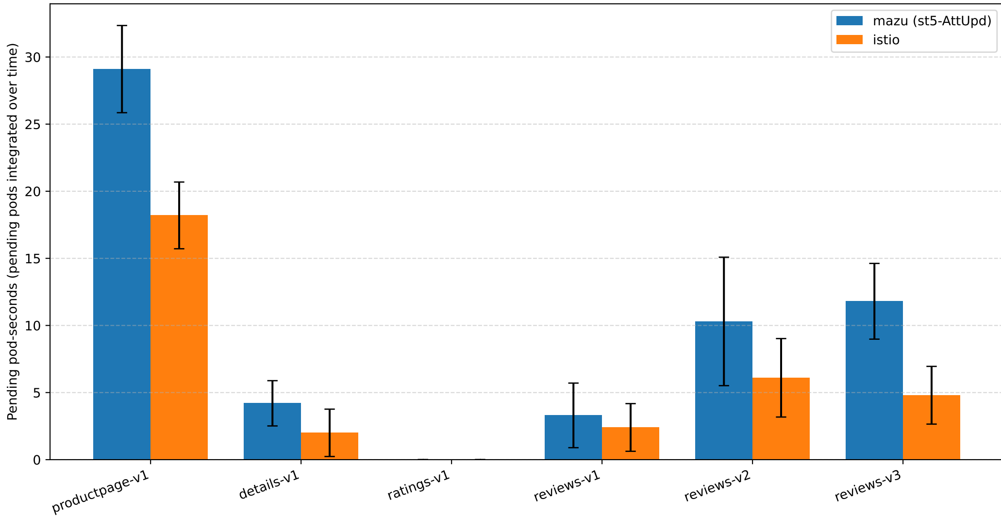
Total pending pod-seconds per service at 400 RPS: mazu (st5-AttUpd) vs istio (mean +/- 1 sigma over runs)
