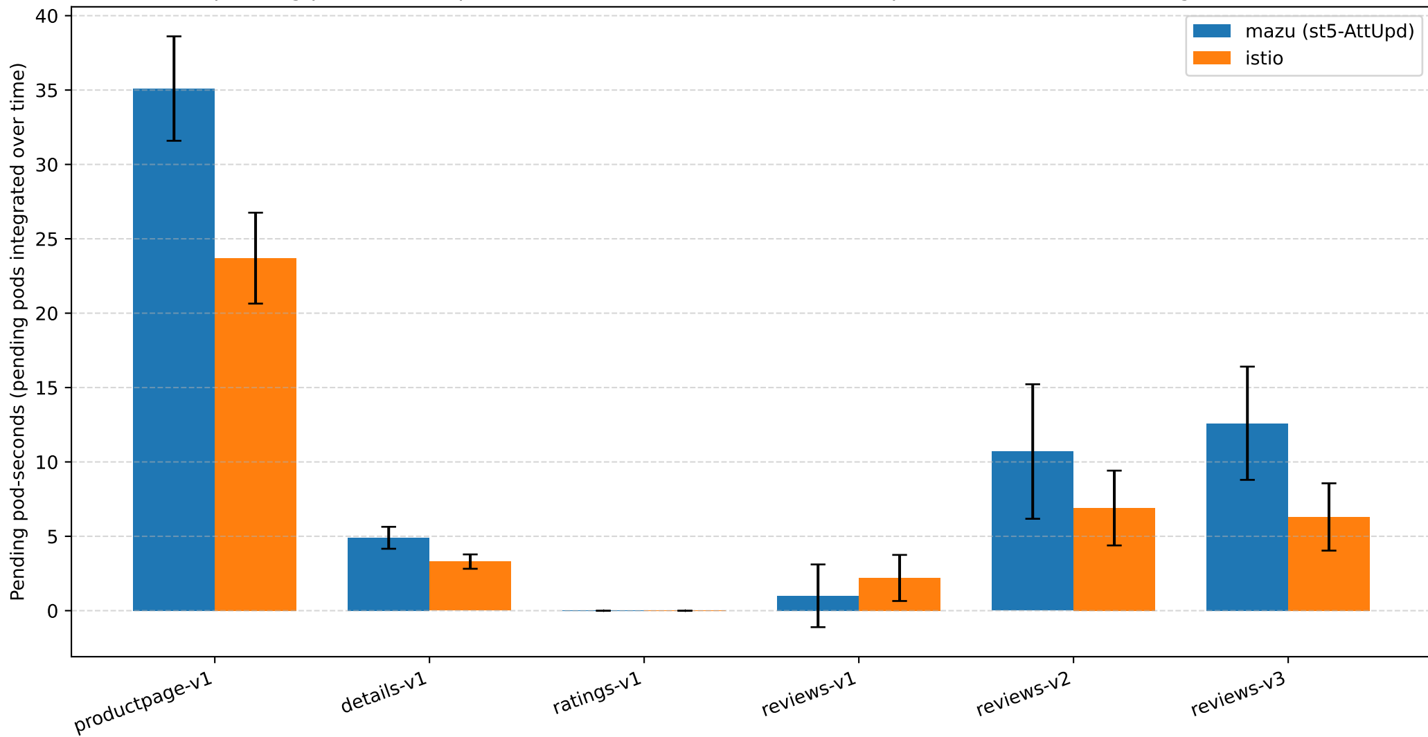
Total pending pod-seconds per service at 500 RPS: mazu (st5-AttUpd) vs istio (mean +/- 1 sigma over runs)
