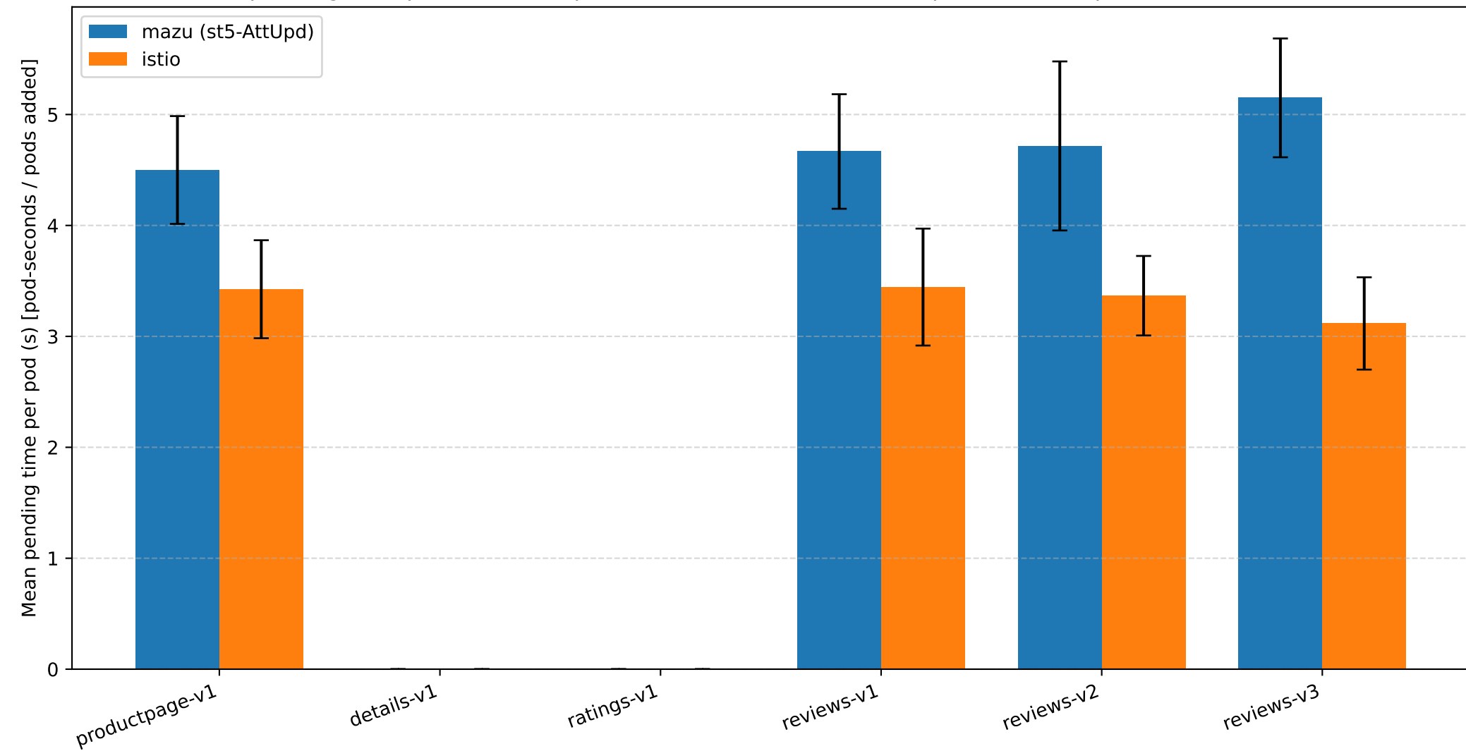
Mean pending time per scheduled pod at 300 RPS: mazu (st5-AttUpd) vs istio (replica-count normalized)
