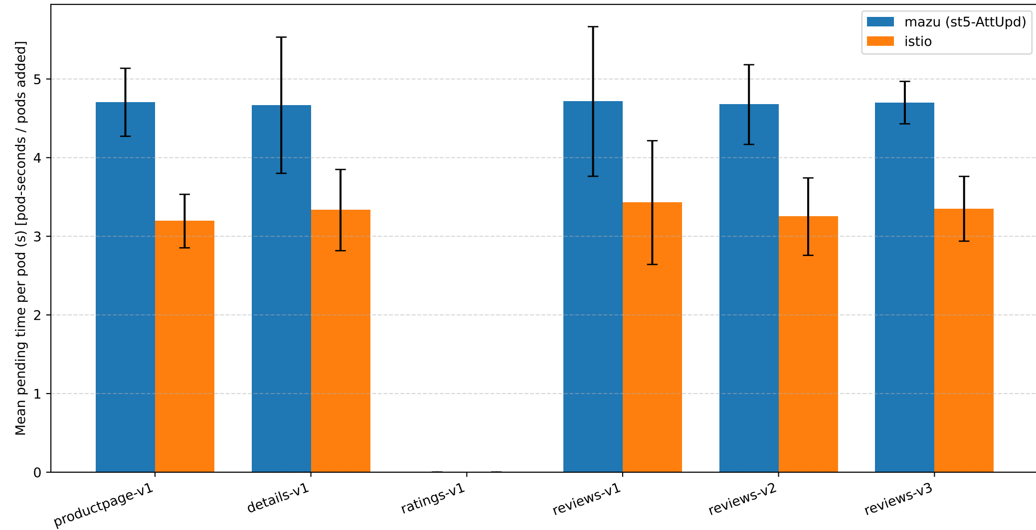
Mean pending time per scheduled pod at 400 RPS: mazu (st5-AttUpd) vs istio (replica-count normalized)
