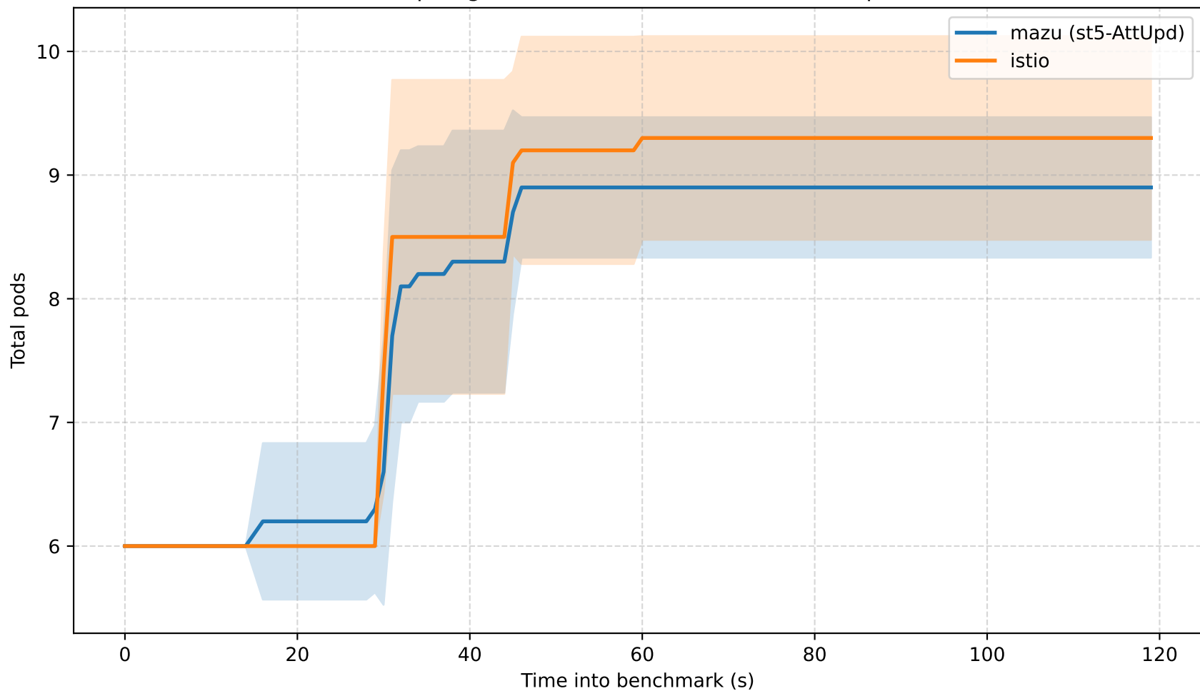
Per-second pod growth at 100 RPS: mazu (st5-AttUpd) vs istio
