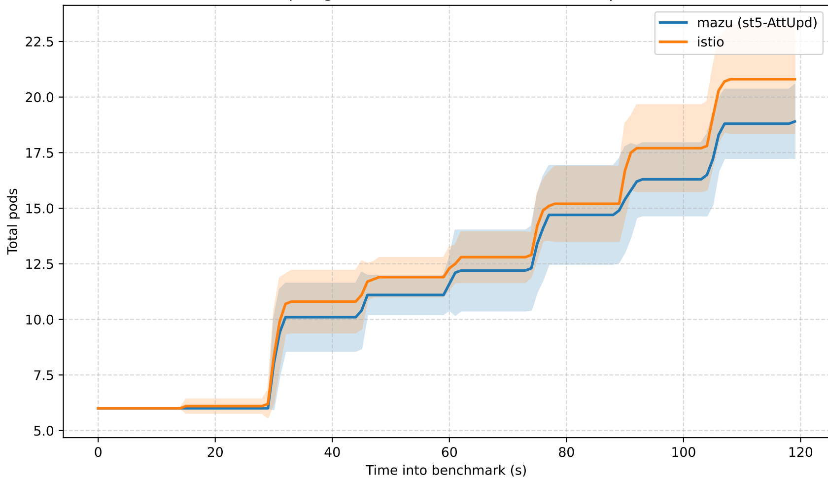
Per-second pod growth at 1100 RPS: mazu (st5-AttUpd) vs istio
