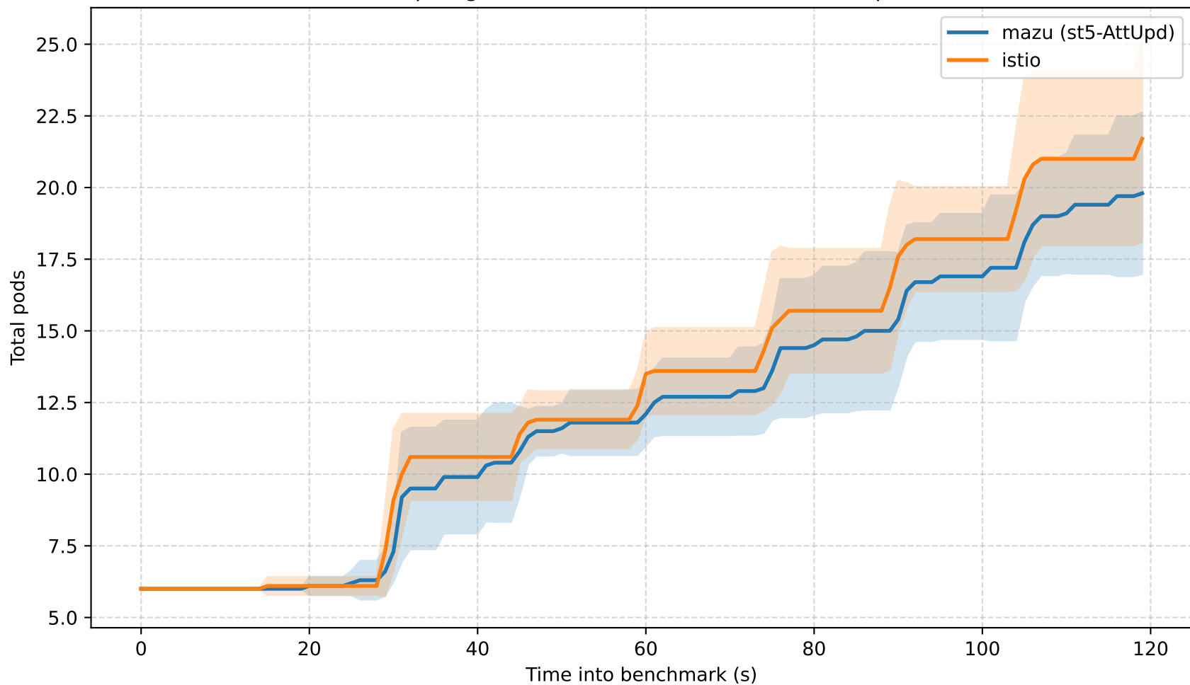
Per-second pod growth at 1200 RPS: mazu (st5-AttUpd) vs istio
