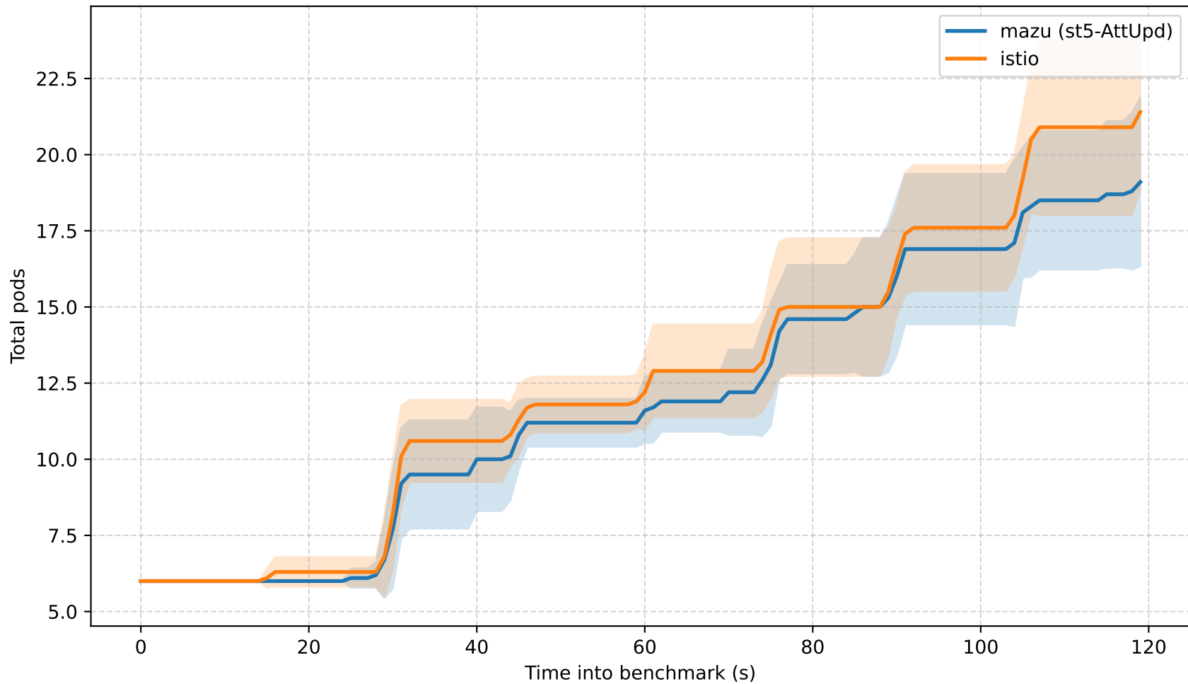
Per-second pod growth at 800 RPS: mazu (st5-AttUpd) vs istio
