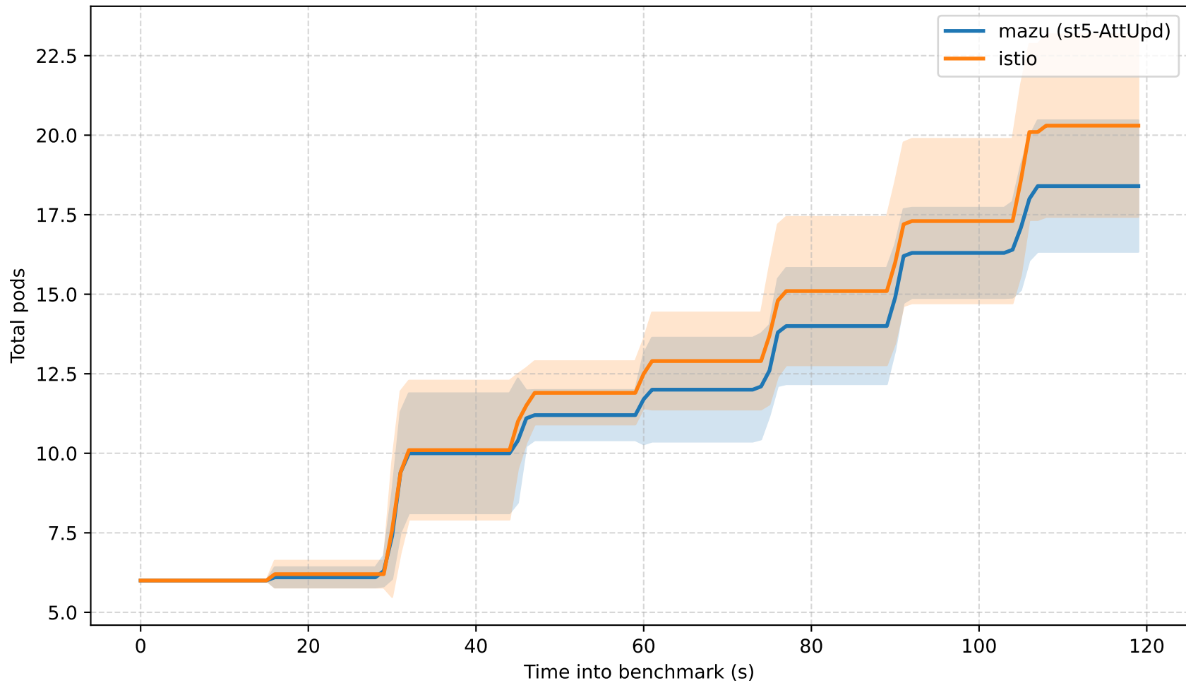
Per-second pod growth at 900 RPS: mazu (st5-AttUpd) vs istio
