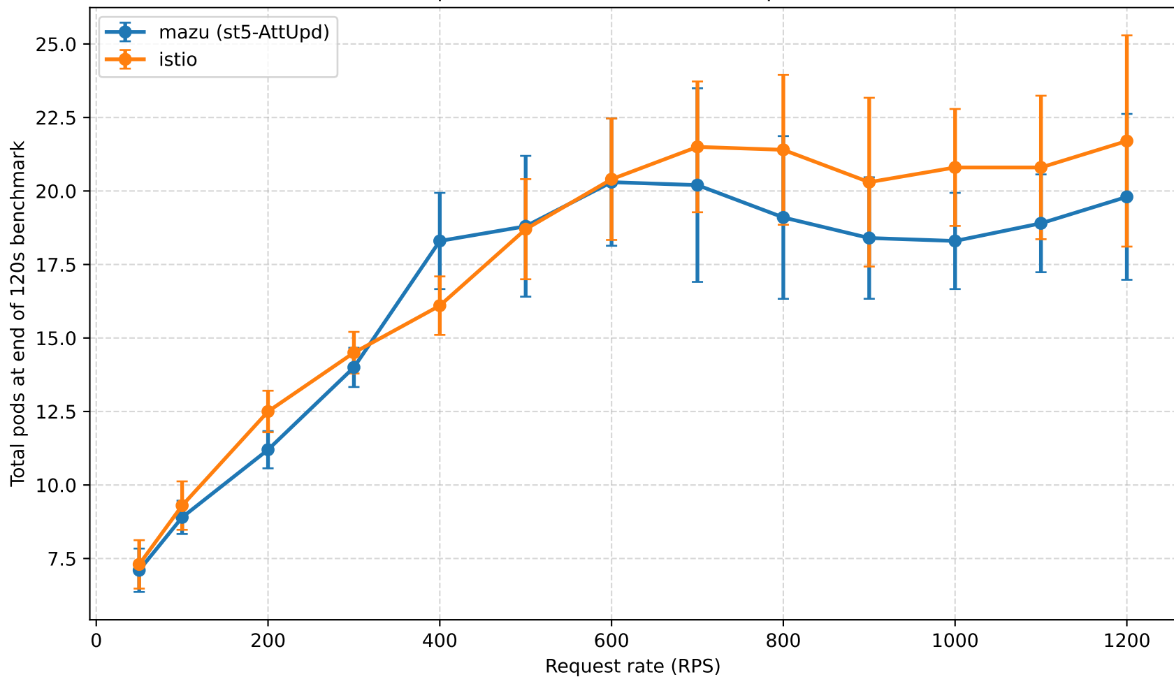
Total pods created: mazu (st5-AttUpd) vs istio
