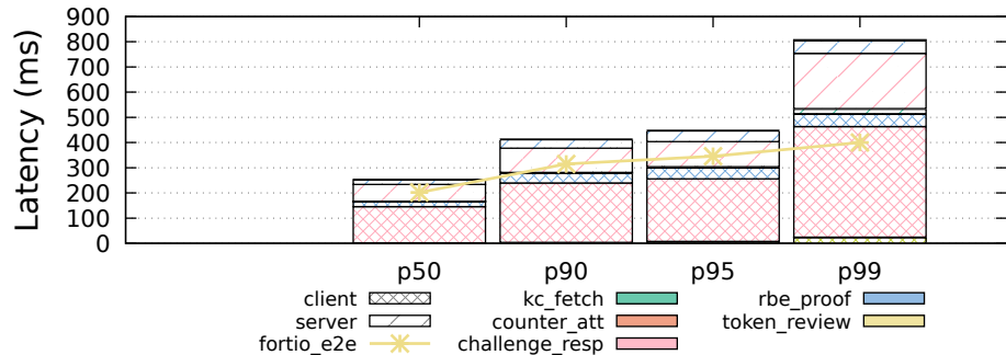
Mazu Latency Breakdown by Operation (50 RPS, 4min)
