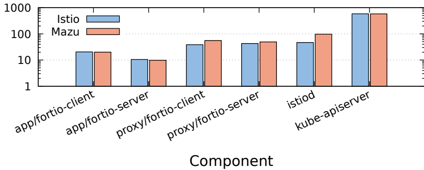
Memory Usage: Istio vs Mazu (50 RPS, 4min)
