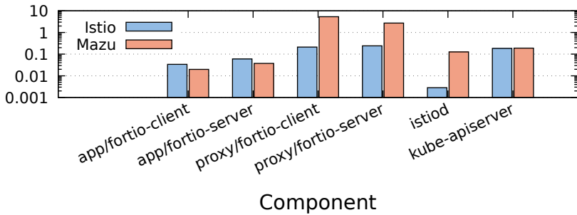
CPU Usage: Istio vs Mazu (50 RPS, 4min, avg of 10 runs)
