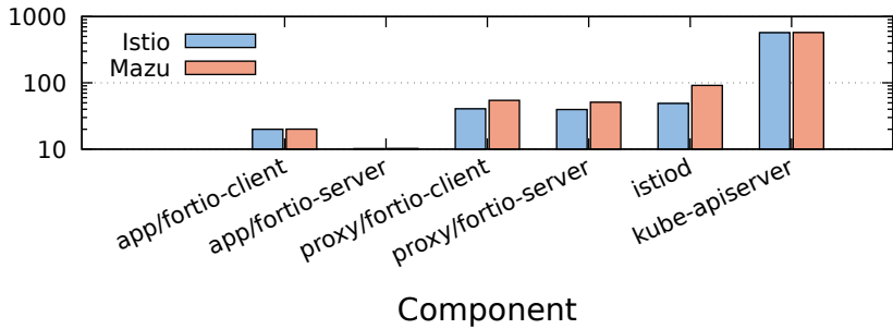
Memory Usage: Istio vs Mazu (50 RPS, 4min, avg of 10 runs)
