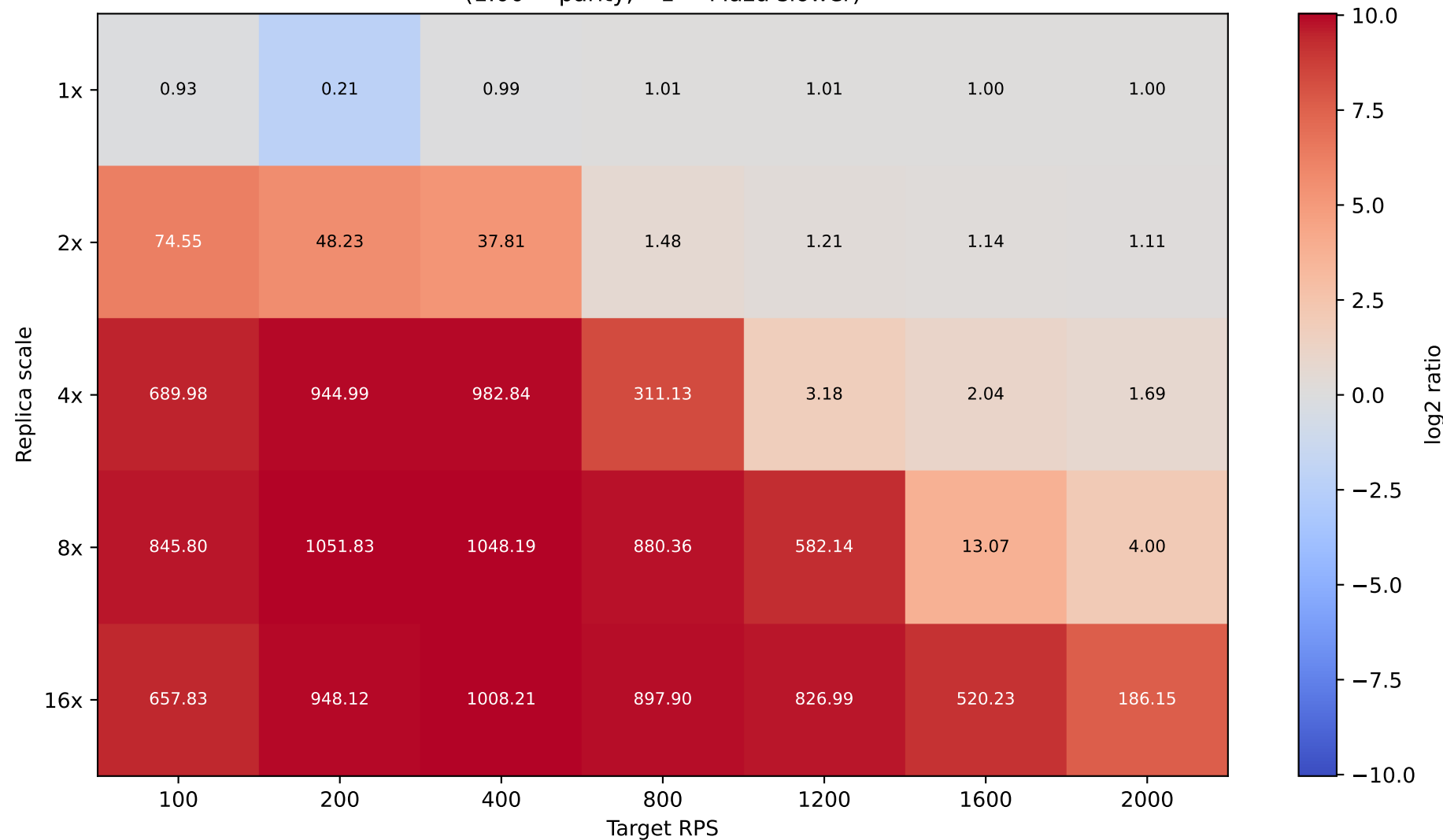
Mazu / Istio p99 latency (1.00 = parity, >1 = Mazu slower)
