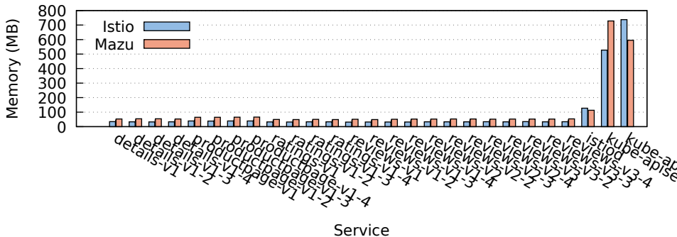
Memory Usage: Istio vs Mazu (800 QPS)
