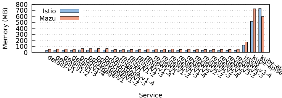
Memory Usage: Istio vs Mazu (200 QPS)
