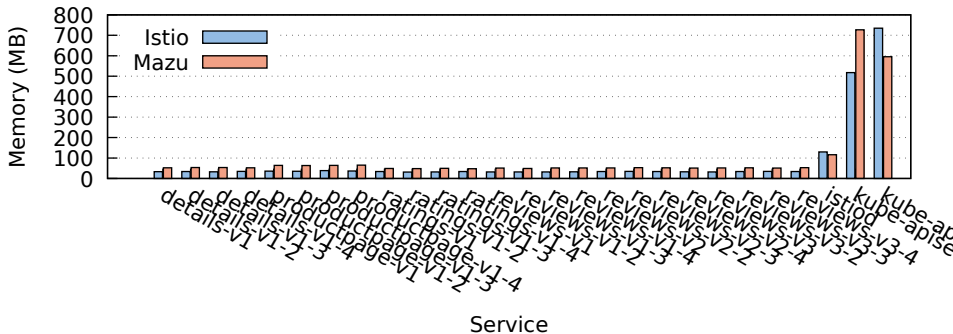
Memory Usage: Istio vs Mazu (400 QPS)
