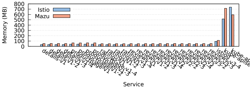
Memory Usage: Istio vs Mazu (1200 QPS)
