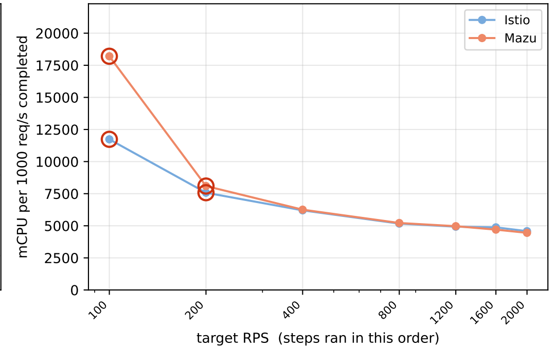
Cost per unit of delivered load (flat = replication is free; rising = it is not)
