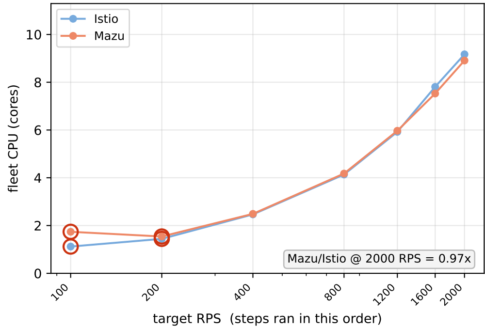
Total mesh CPU (istio-proxy sidecars + istiod)
