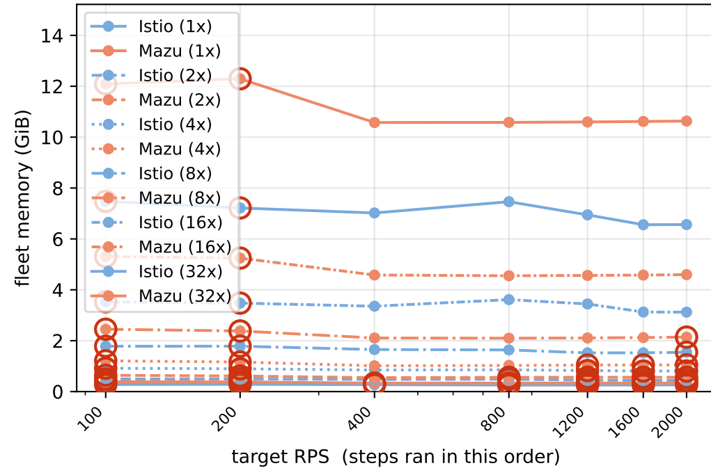
Total mesh memory (istio-proxy sidecars + istiod)
