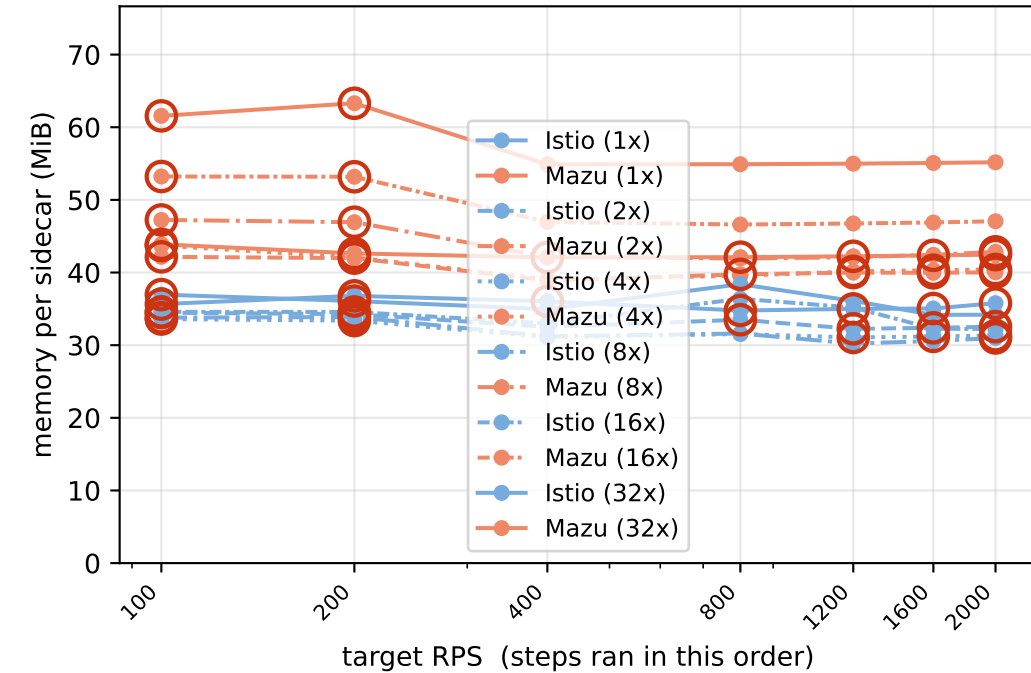
Per-sidecar footprint (fleet memory / sidecar count)
