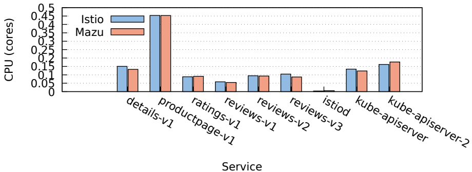
CPU Usage: Istio vs Mazu (1200 QPS)
