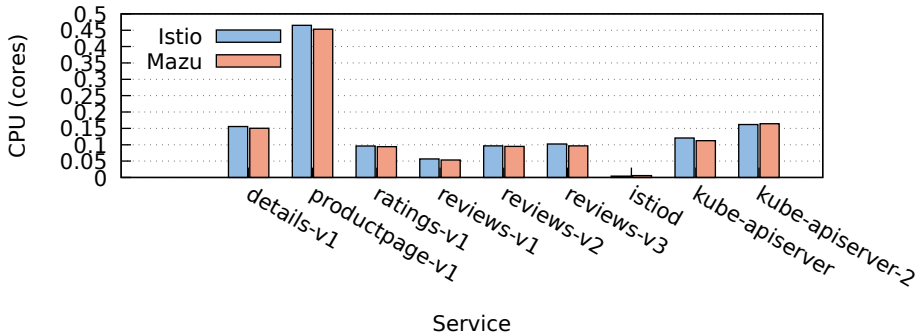
CPU Usage: Istio vs Mazu (1600 QPS)
