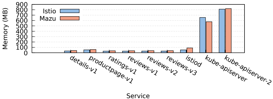
Memory Usage: Istio vs Mazu (1200 QPS)
