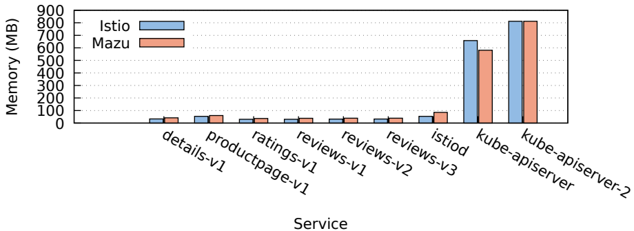
Memory Usage: Istio vs Mazu (1600 QPS)
