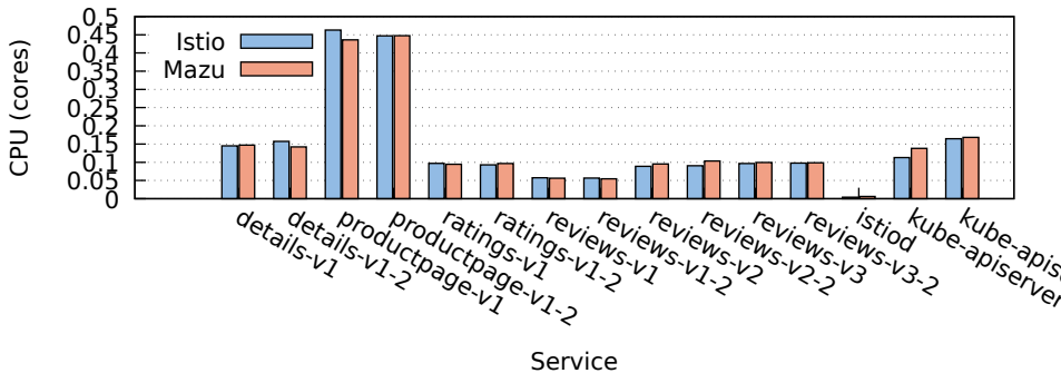
CPU Usage: Istio vs Mazu (1200 QPS)
