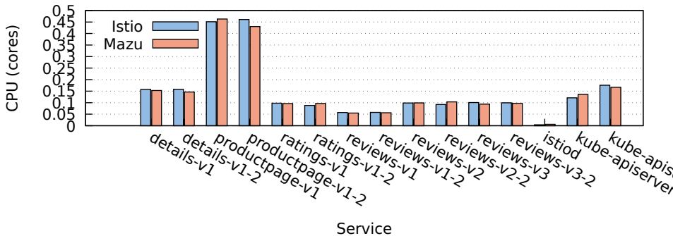
CPU Usage: Istio vs Mazu (1600 QPS)
