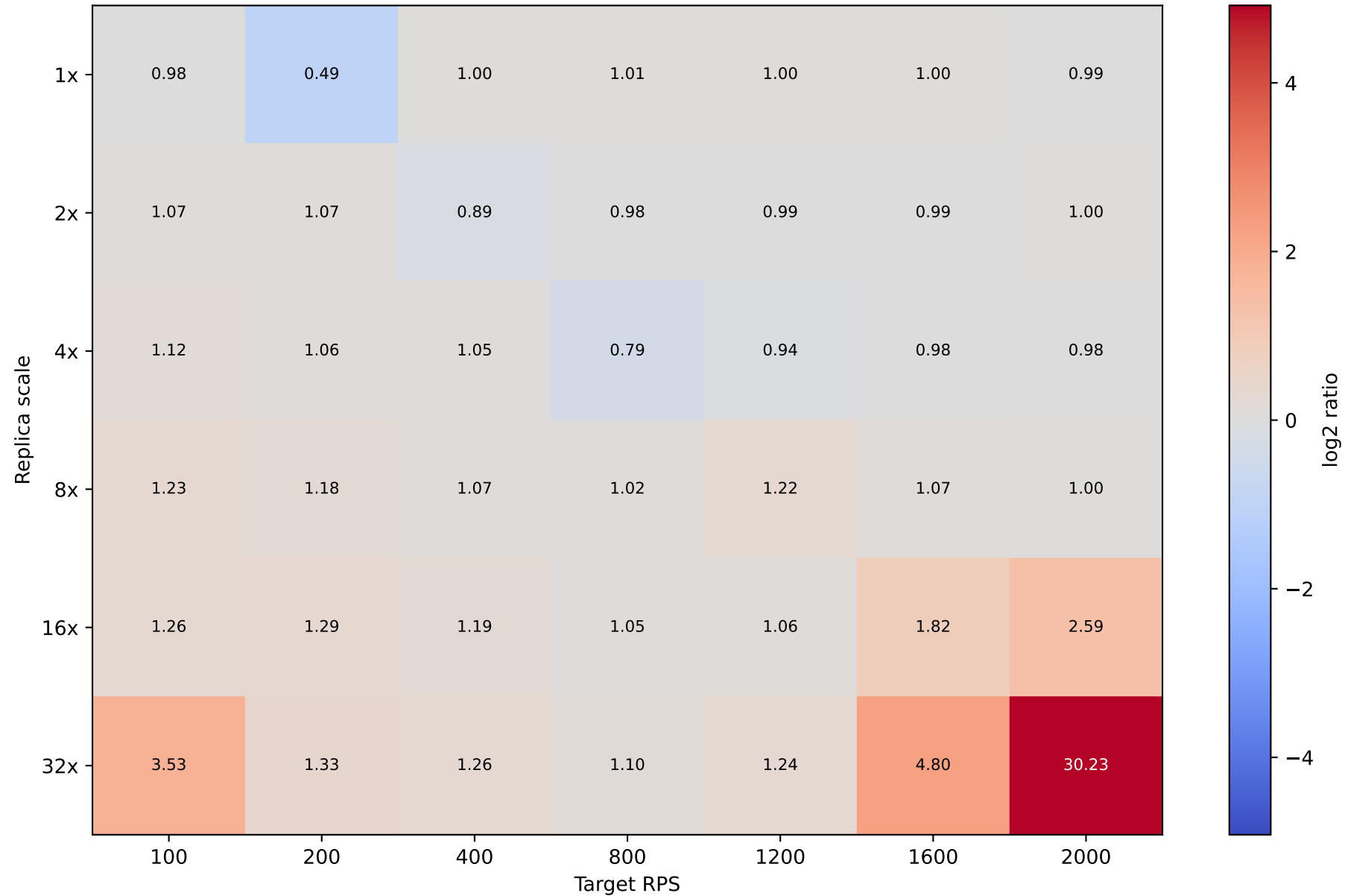
Mazu / Istio p99 latency (1.00 = parity, >1 = Mazu slower)
