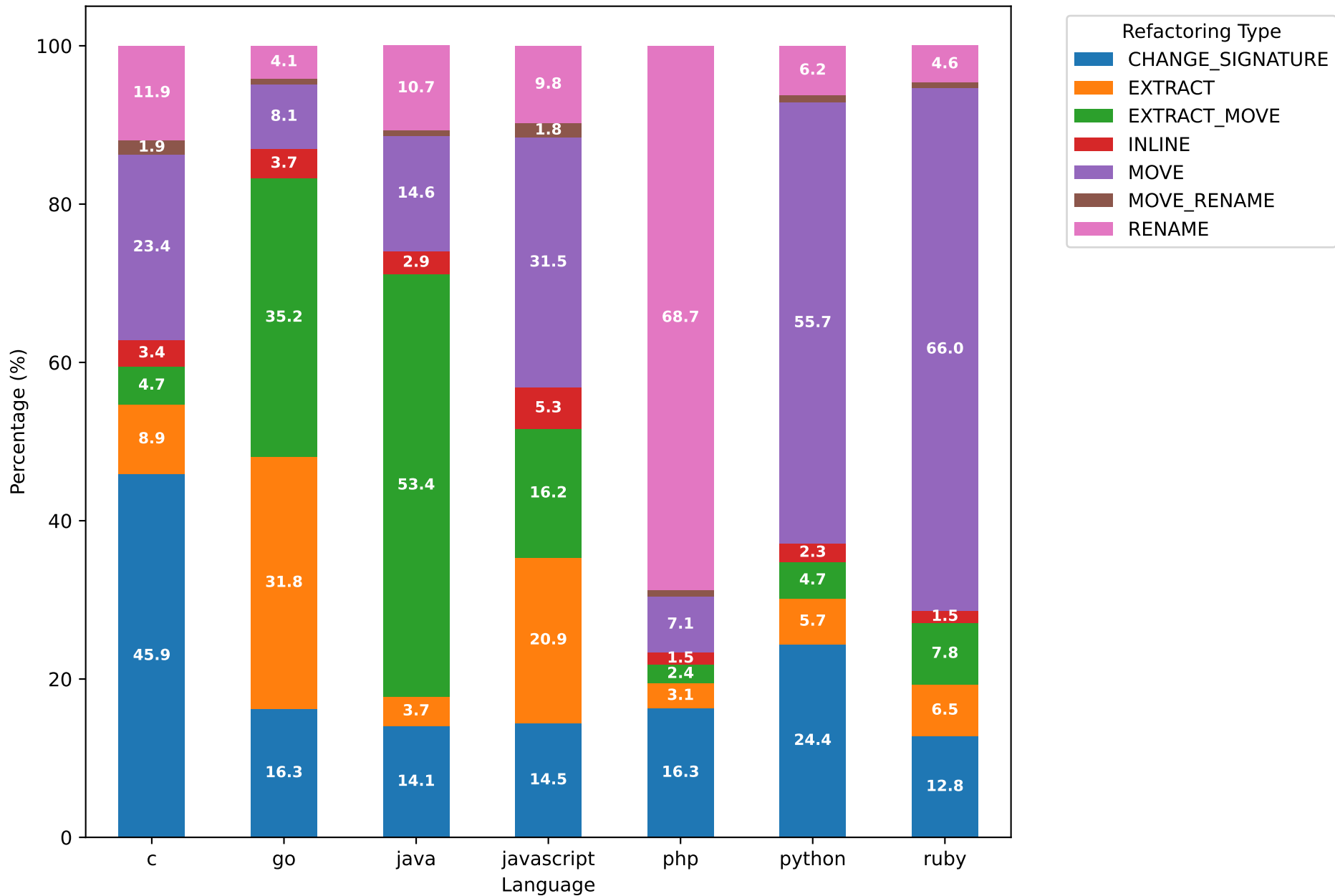
Distribution of Refactoring Types by Language
