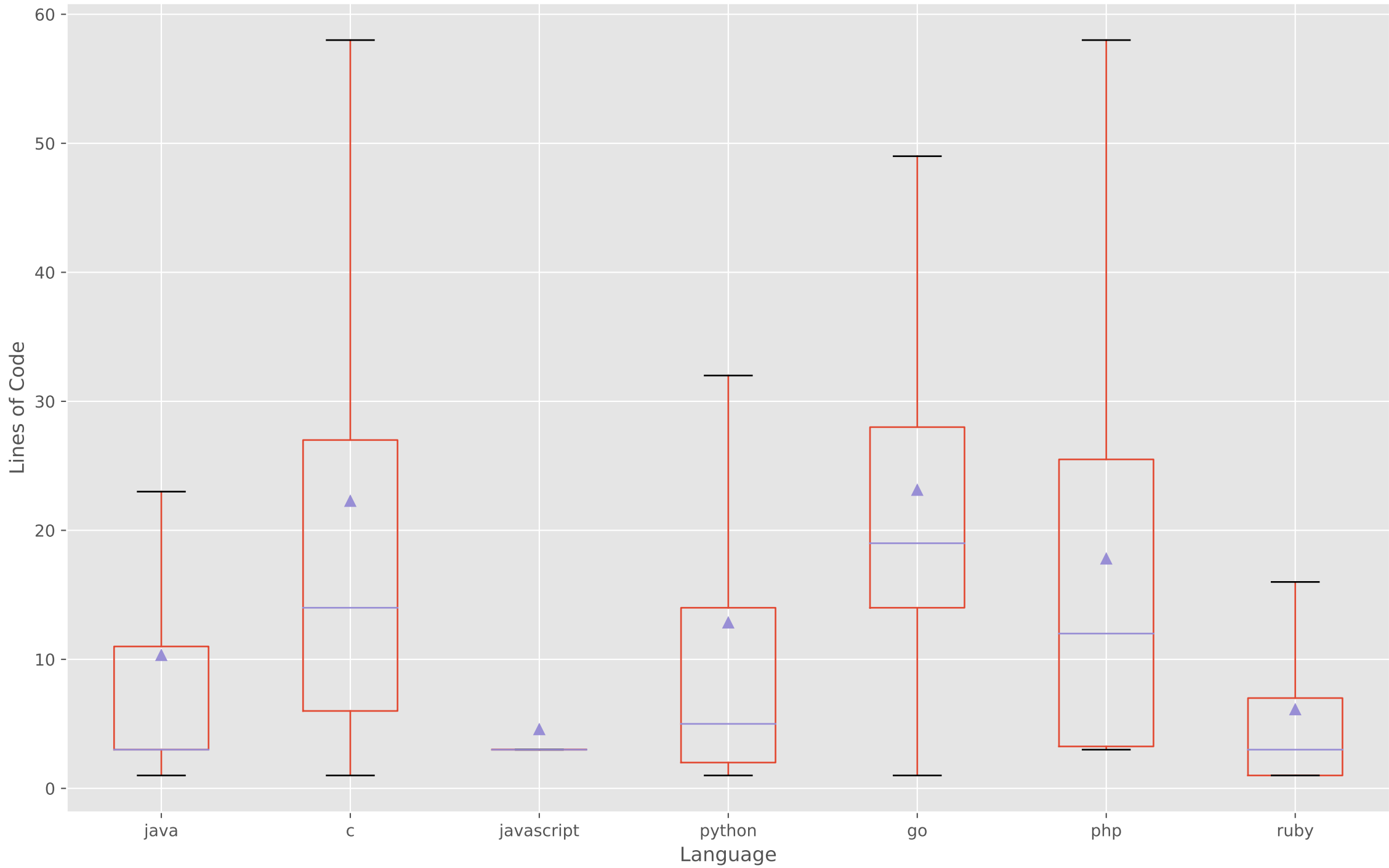
AfterLOC for EXTRACT Refactoring by Language
