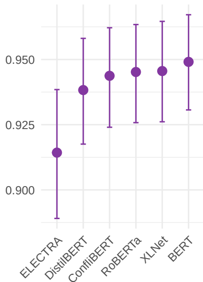
b. CIs at 25% Training
