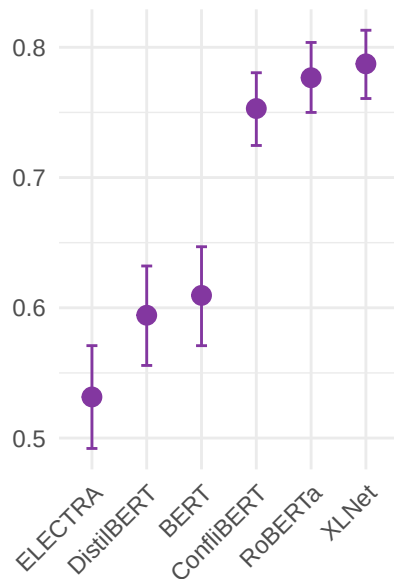
b. CIs at 25% Training
