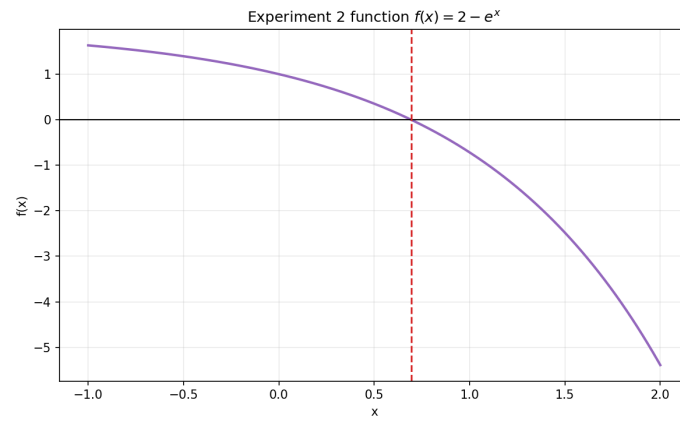
Figure 3: Experiment 2 function f(x) = 2 - e^x on [-1, 2] .
